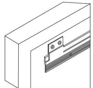
Z-Clip/Z-Rail
